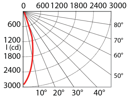
PHOTOMETRIC CURVE
