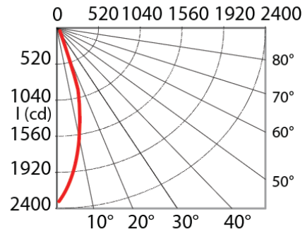
PHOTOMETRIC CURVE
