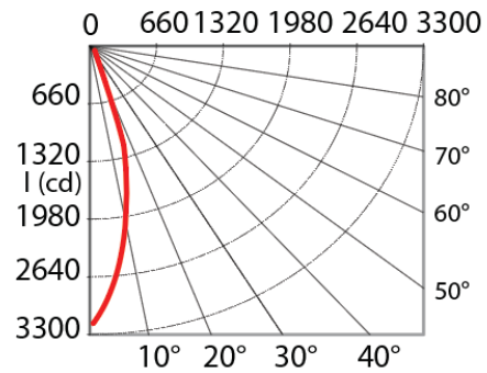
PHOTOMETRIC CURVE
