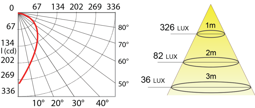
PHOTOMETRIC CURVE BEAM 45° AMPLITUDE DIAGRAM
