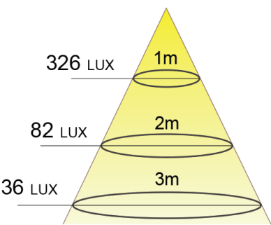
BEAM 45° AMPLITUDE DIAGRAM
