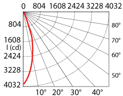
PHOTOMETRIC CURVE
