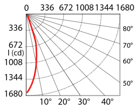
PHOTOMETRIC CURVE
