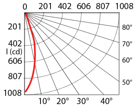
PHOTOMETRIC CURVE
