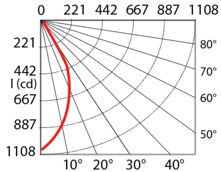
PHOTOMETRIC CURVE
