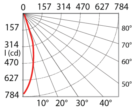
PHOTOMETRIC CURVE
