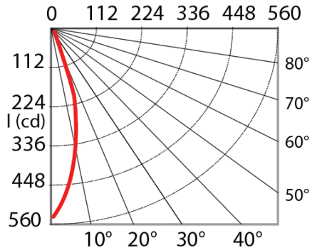
PHOTOMETRIC CURVE
