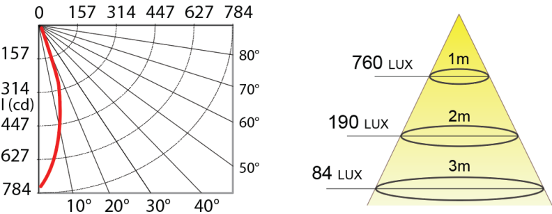
PHOTOMETRIC CURVE BEAM 36° AMPLITUDE DIAGRAM
