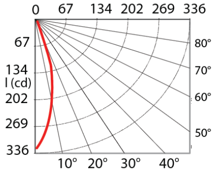
PHOTOMETRIC CURVE
