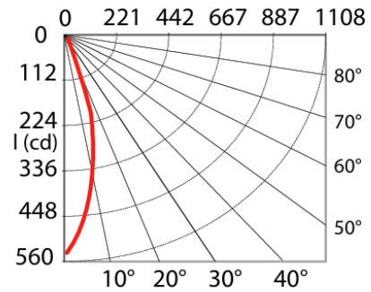
PHOTOMETRIC CURVE
