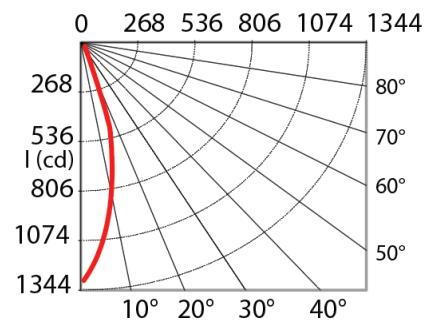
PHOTOMETRIC CURVE
