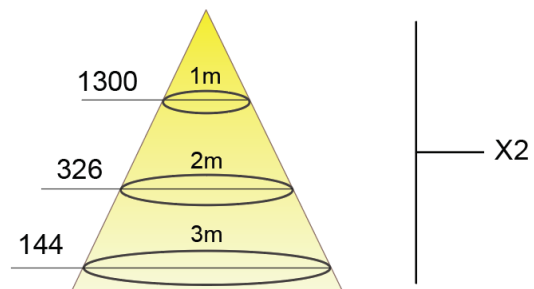
BEAM 36° AMPLITUDE DIAGRAM
