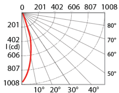
PHOTOMETRIC CURVE
