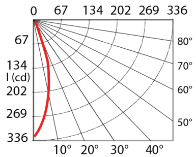
PHOTOMETRIC CURVE
