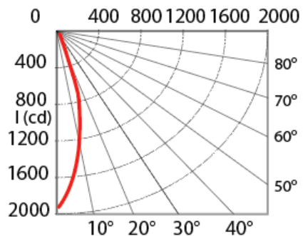
PHOTOMETRIC CURVE
