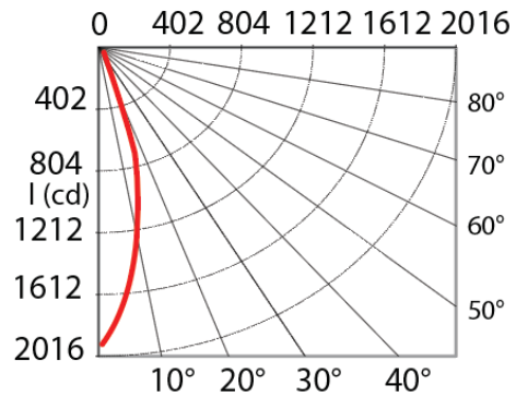
PHOTOMETRIC CURVE
