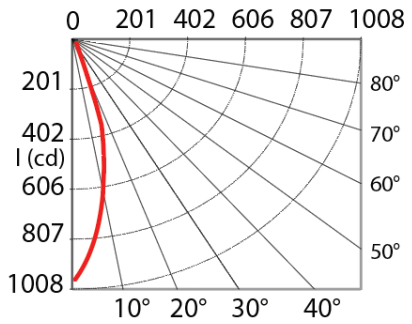
PHOTOMETRIC CURVE
