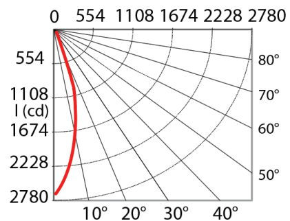
PHOTOMETRIC CURVE
