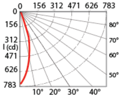
PHOTOMETRIC CURVE
