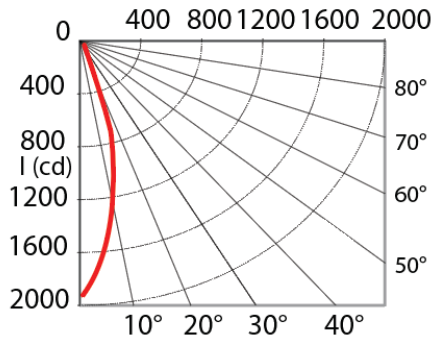
PHOTOMETRIC CURVE
