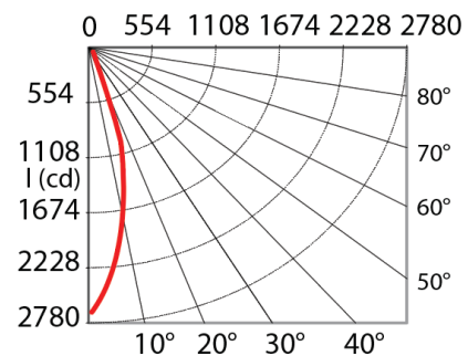
PHOTOMETRIC CURVE
