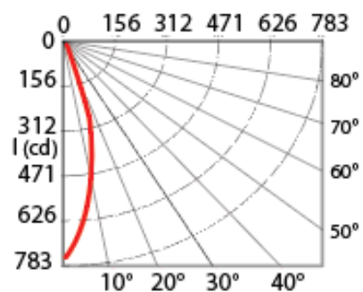
PHOTOMETRIC CURVE
