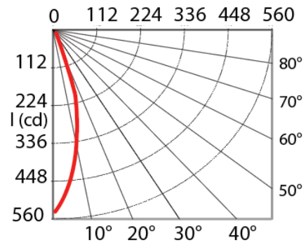
PHOTOMETRIC CURVE
