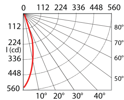
PHOTOMETRIC CURVE
