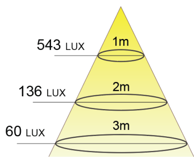
BEAM 36° AMPLITUDE DIAGRAM
