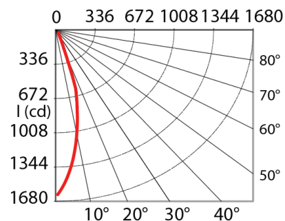
PHOTOMETRIC CURVE
