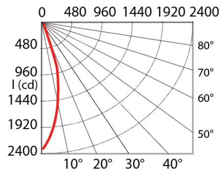
PHOTOMETRIC CURVE
