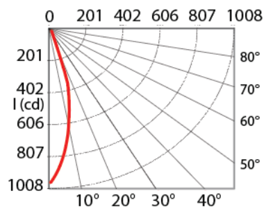
PHOTOMETRIC CURVE
